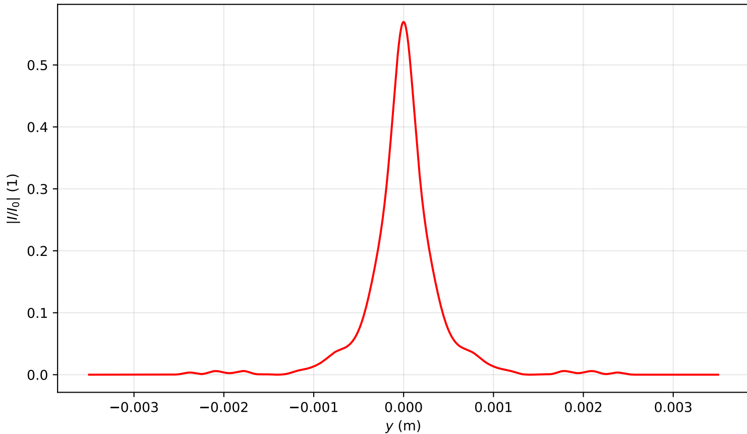
Intensity profile I(x=0, y, z=2.548)/I_0 , P_{in}=4.0P_{cr} , artificial time
